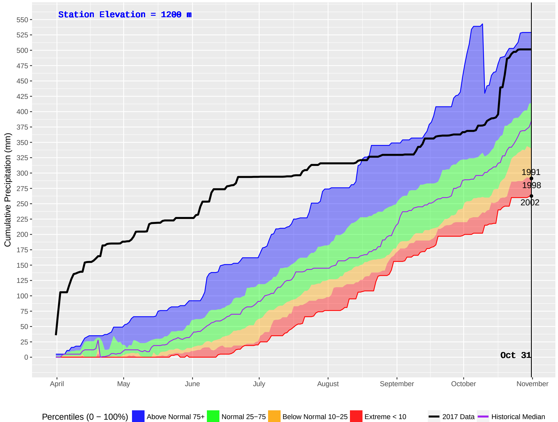
TSAR CREEK (361) : Historical (1986–2016) and Current (2017) Noon Cumulative Precipitation
