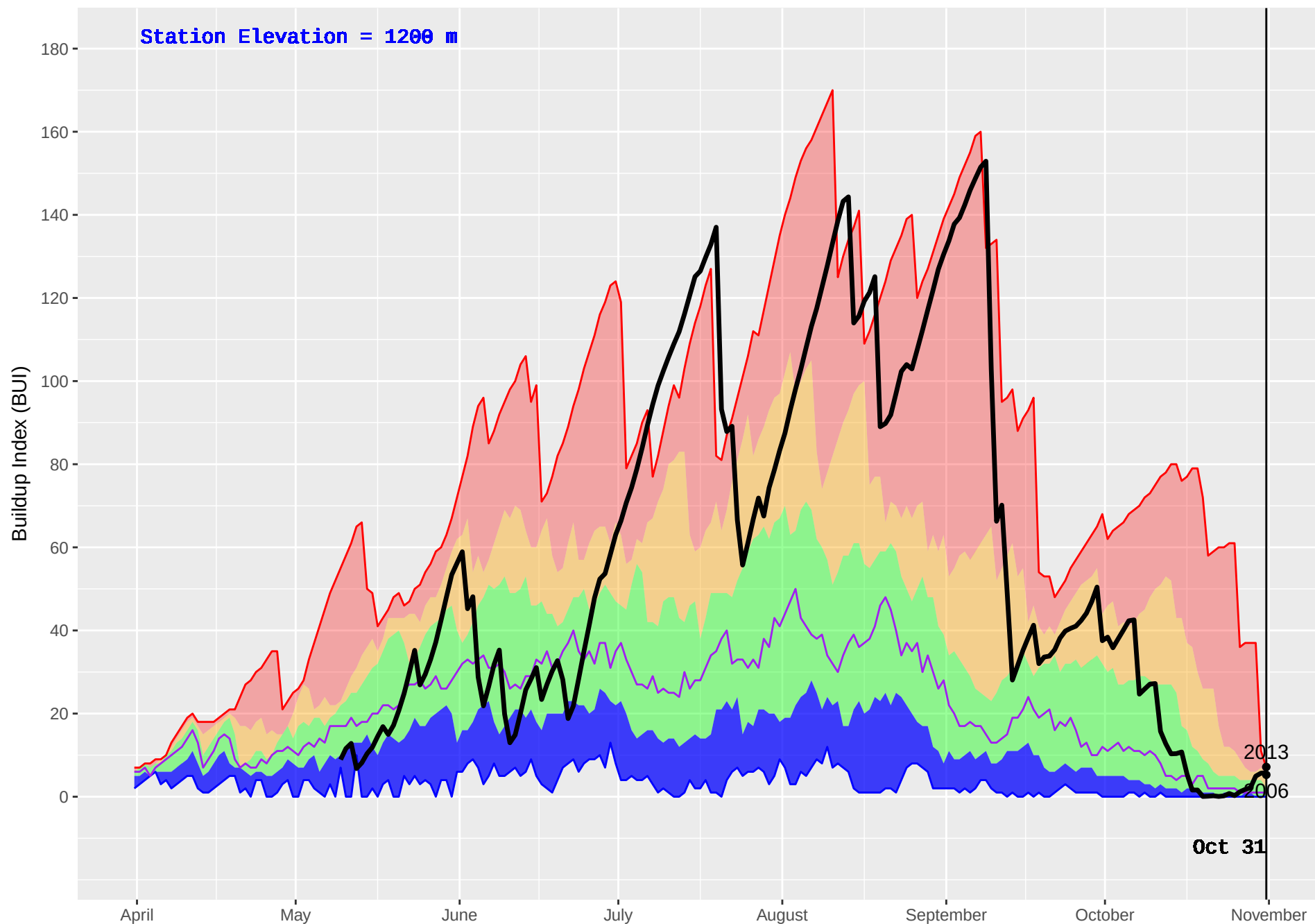
TSAR CREEK (361) : Historical (1986–2016) and Current (2017) Noon Buildup Index (BUI)
