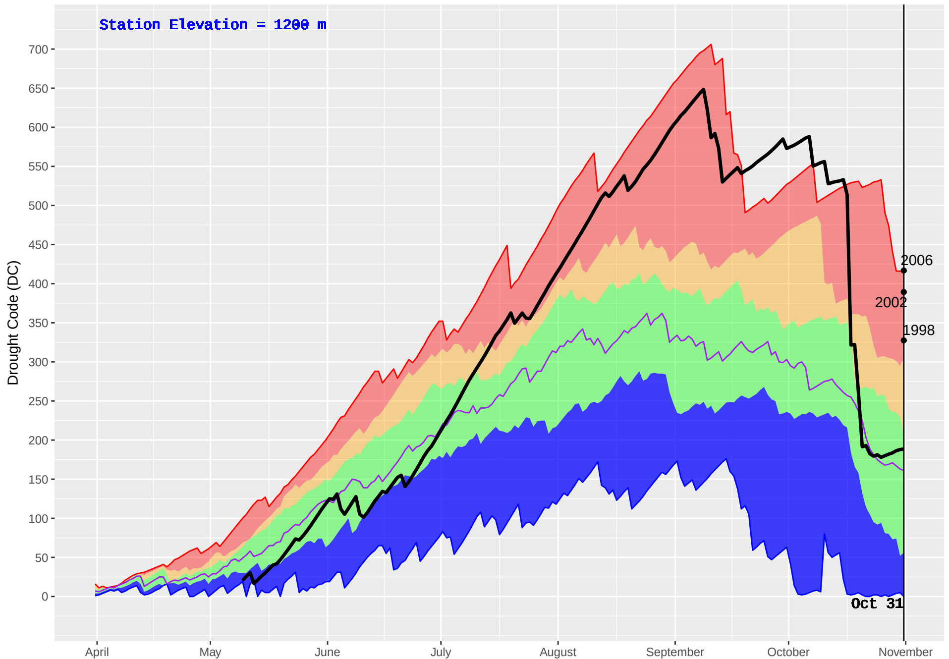
TSAR CREEK (361) : Historical (1986–2016) and Current (2017) Noon Drought Code (DC)
